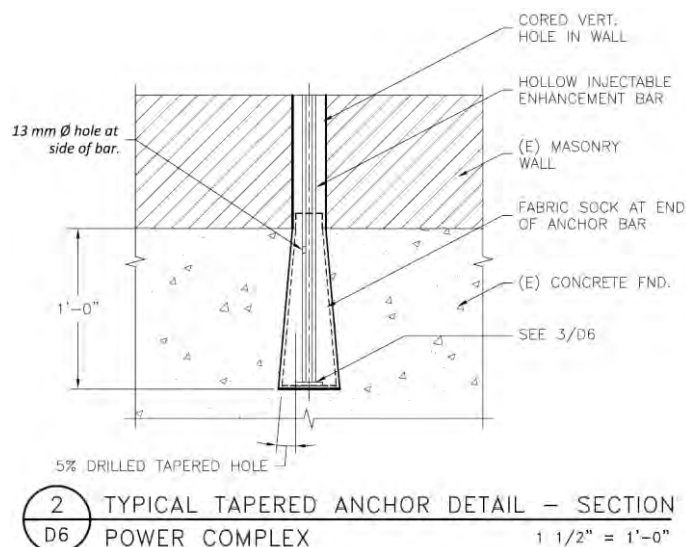
Fig. 5 Left, design detail showing the reverse tapered vertical reinforcing termination. Right, installed taper.
