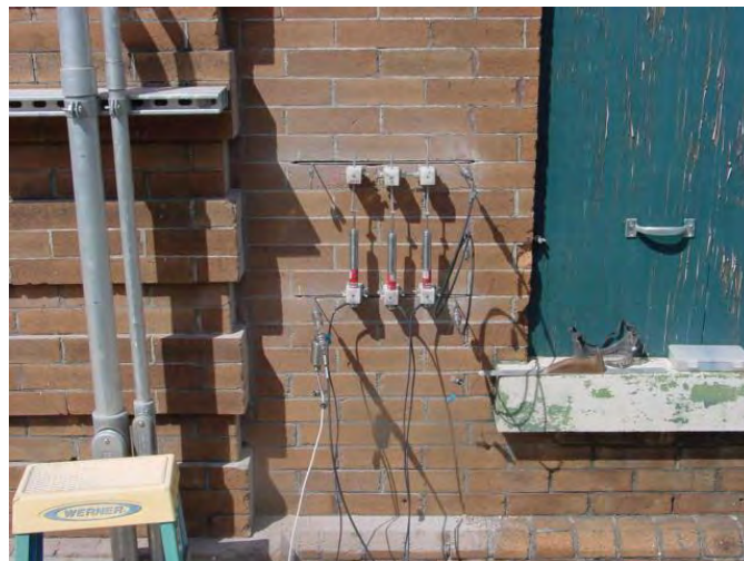
Fig. 4 Flatjack testing at Pump Station 7 to determine existing masonry compressive strength and stiffness.
